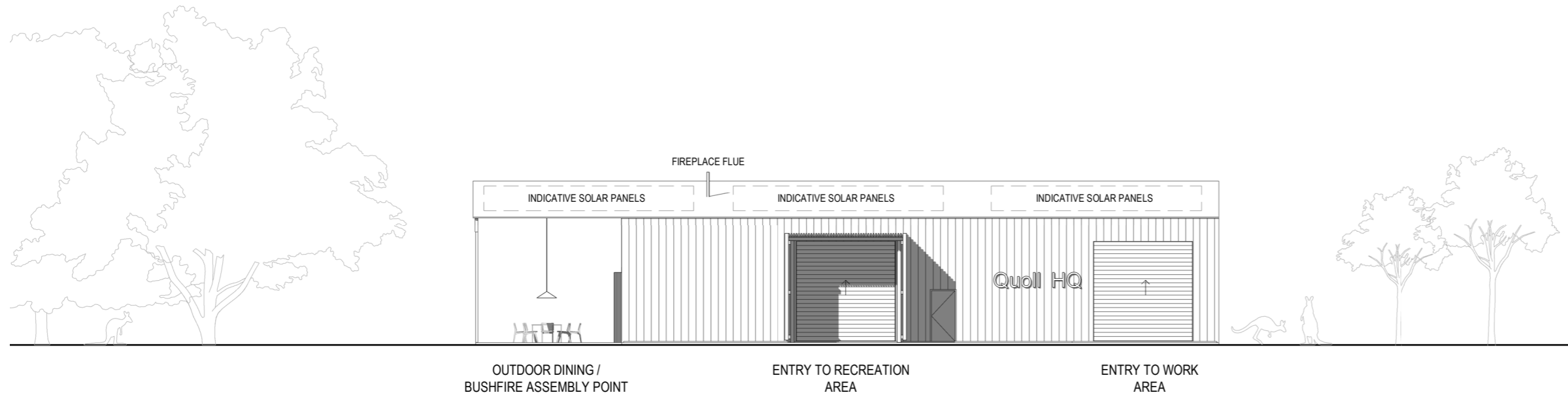
PROPOSED ELEVATION 02 1:200
